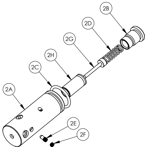
ITEM 2, VALVE ASSEMBLY
